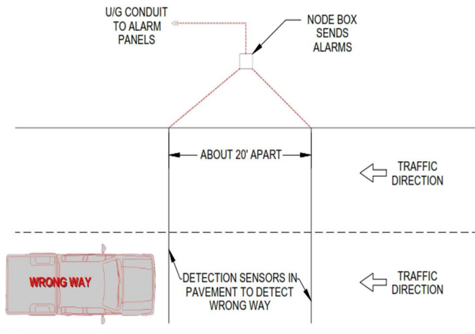
WRONG WAY DETECTION LAYOUT
